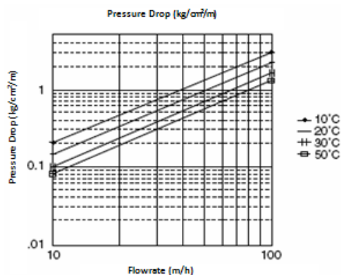
Figure 1: Pressure Drop
